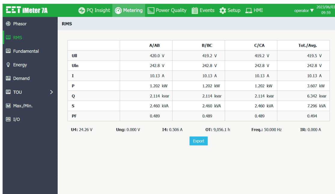
Figure 3-69 RMS Metering
