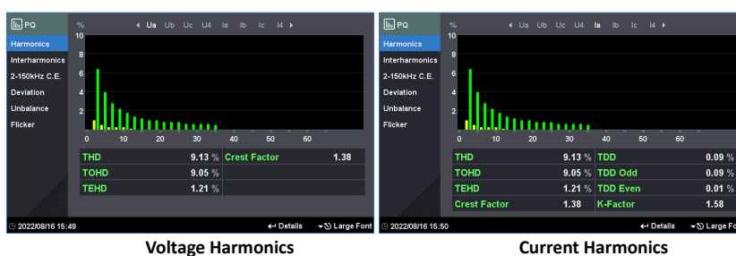
Figure 3-20 Harmonics Overview
