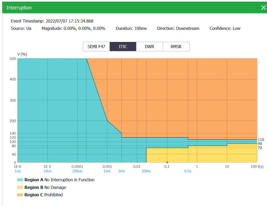
Figure 3-113 Interruption on ITIC Interface
