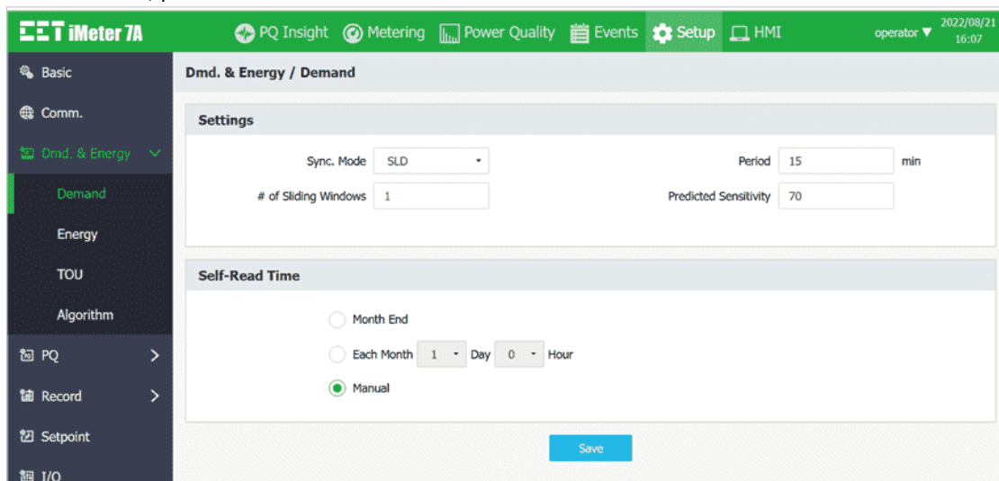
Figure 3-126 Demand Setup Interface
