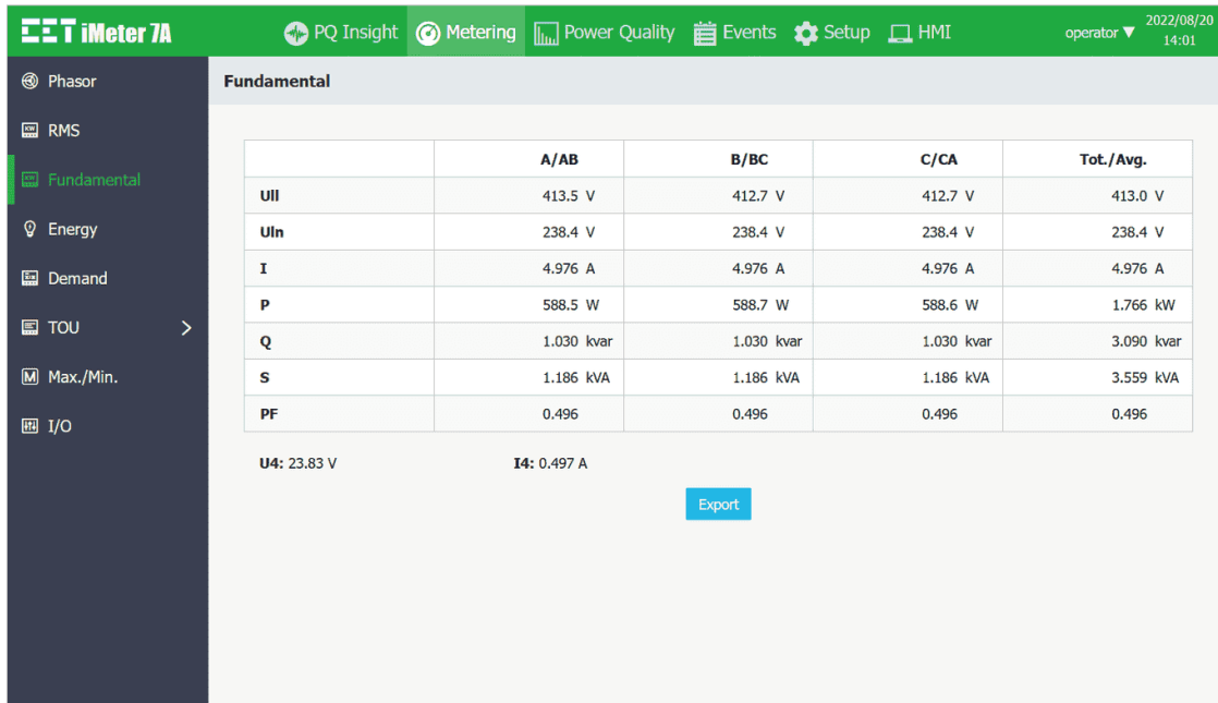
Figure 3-70 Fundamental Metering
