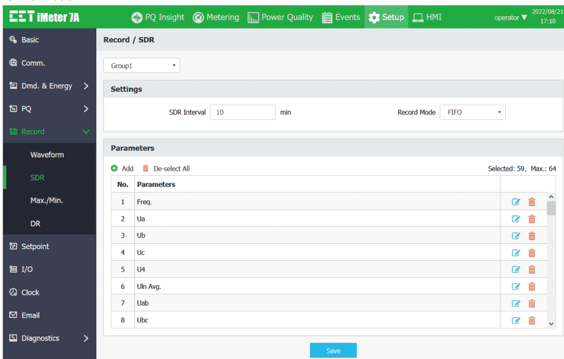
Figure 3-156 SDR Settings Interface
