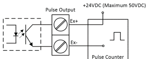
Figure 2-21 Pulse Output (Solid State Relay) Connections for Energy Pulsing
