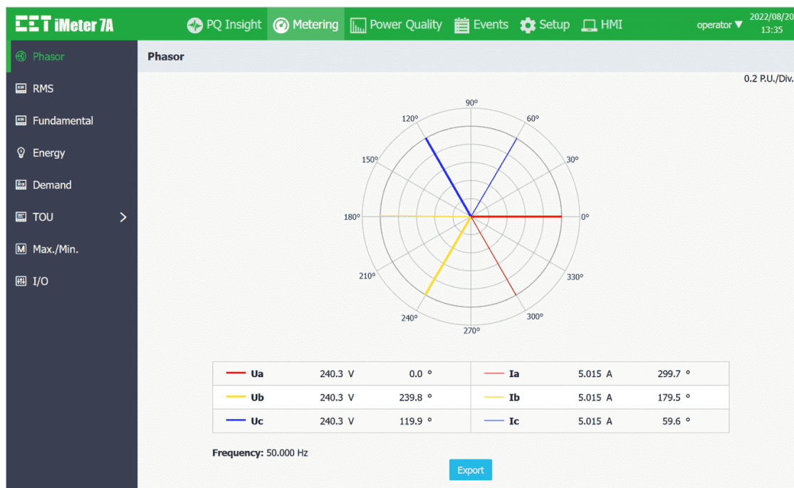
Figure 3-68 Phasor Diagram
