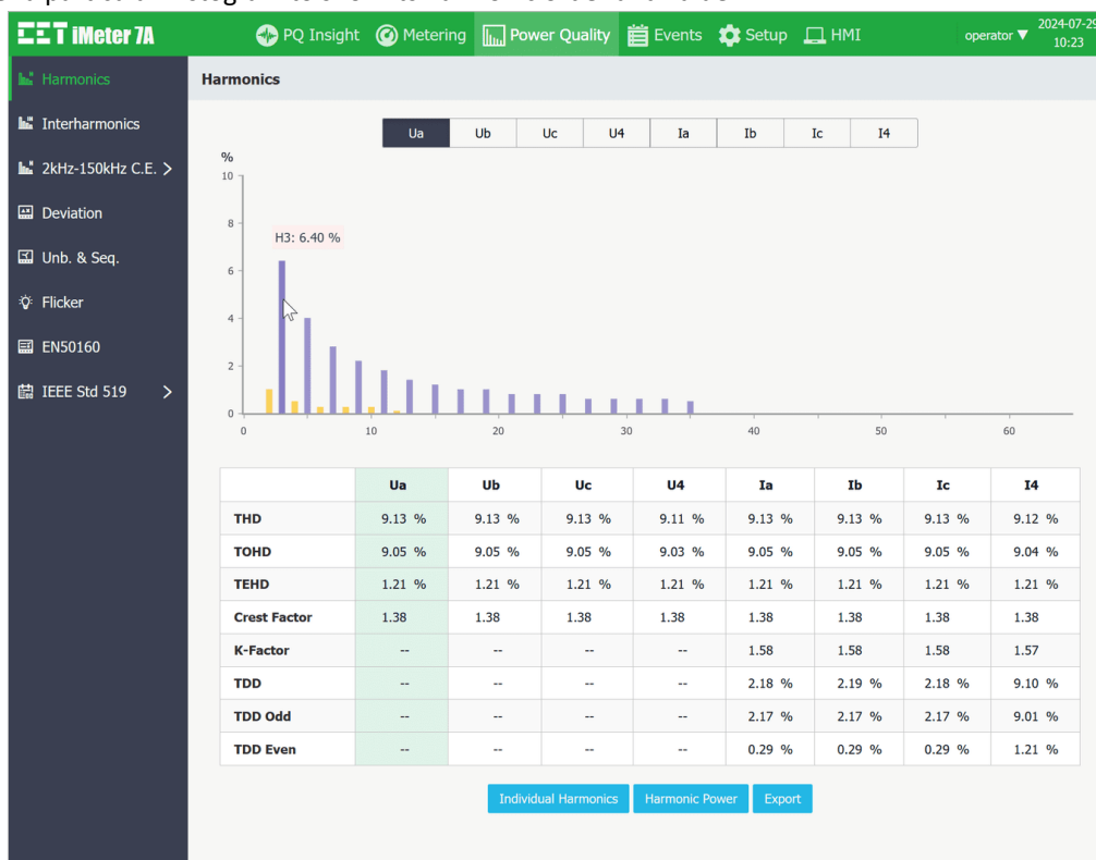
Figure 3-82 Harmonics Interface
