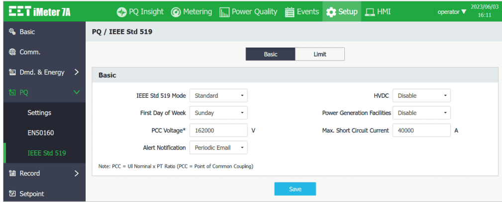
Figure 3-147 IEEE Std 519 Basic Configuration
