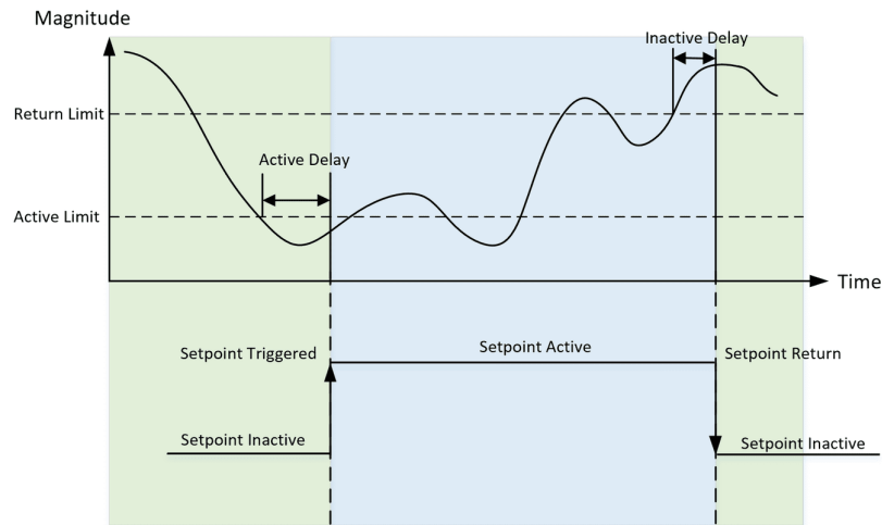
Figure 4-26 Under Setpoint
