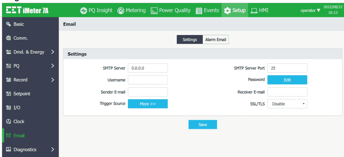
Figure 3-170 Alarm Email Setup Interface
