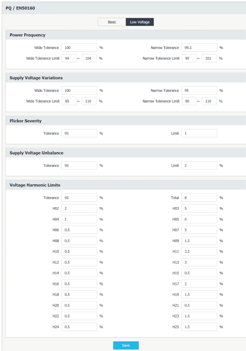
Figure 3-146 Default Limits of the EN 50160 Parameters for Low Voltage
