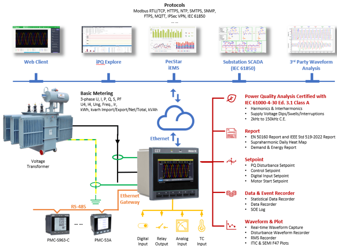
Figure 1-1 Typical Application
