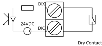
Figure 2-15 DI Connections
