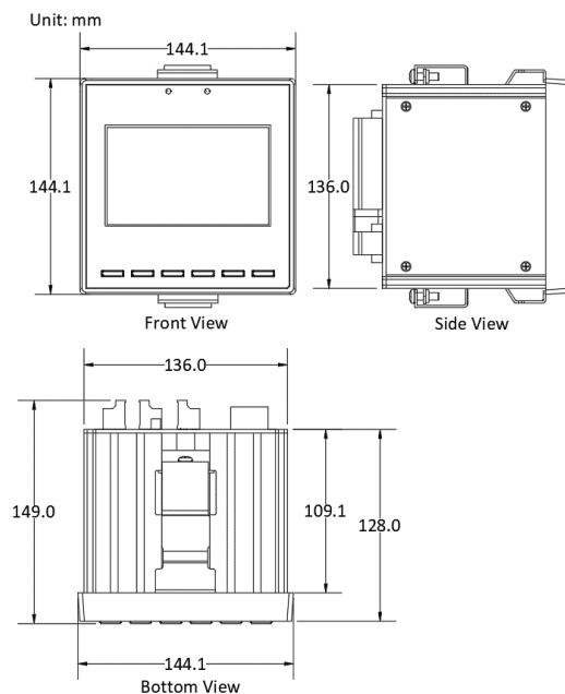
Figure 2-2 Unit Dimension
