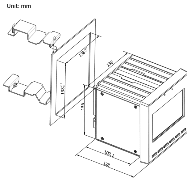
Figure 2-3 Installation
