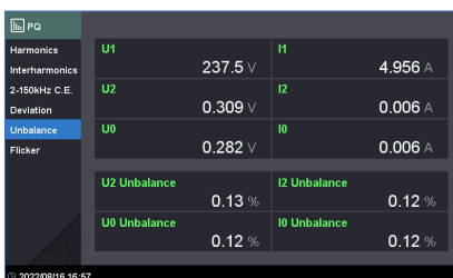
Figure 3-28 Unbalance
