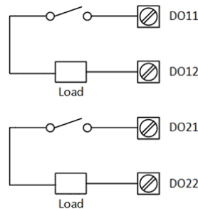
Figure 2-18 DO Connections
