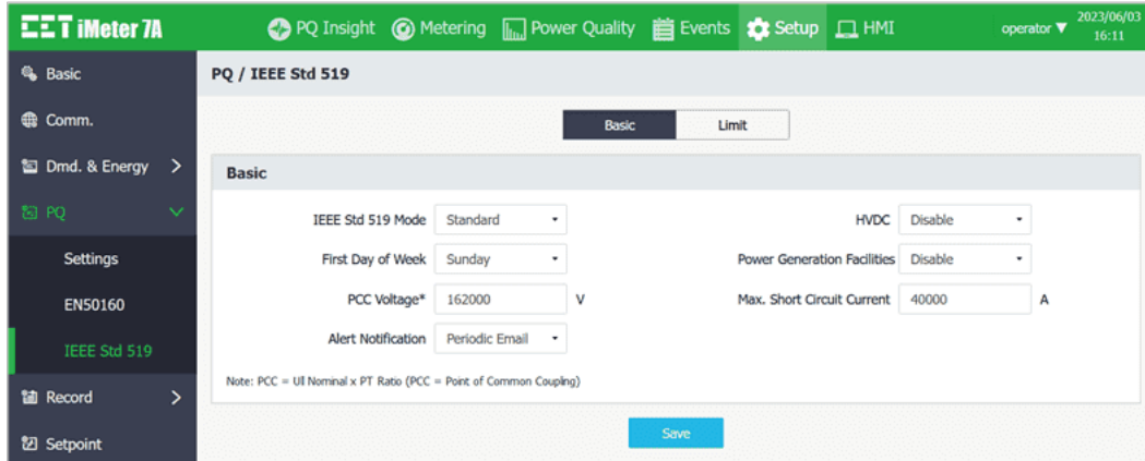
Figure 4-20 IEEE Std 519 Basic Parameters Configuration via Web Interface
