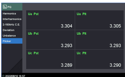
Figure 3-29 Flicker
