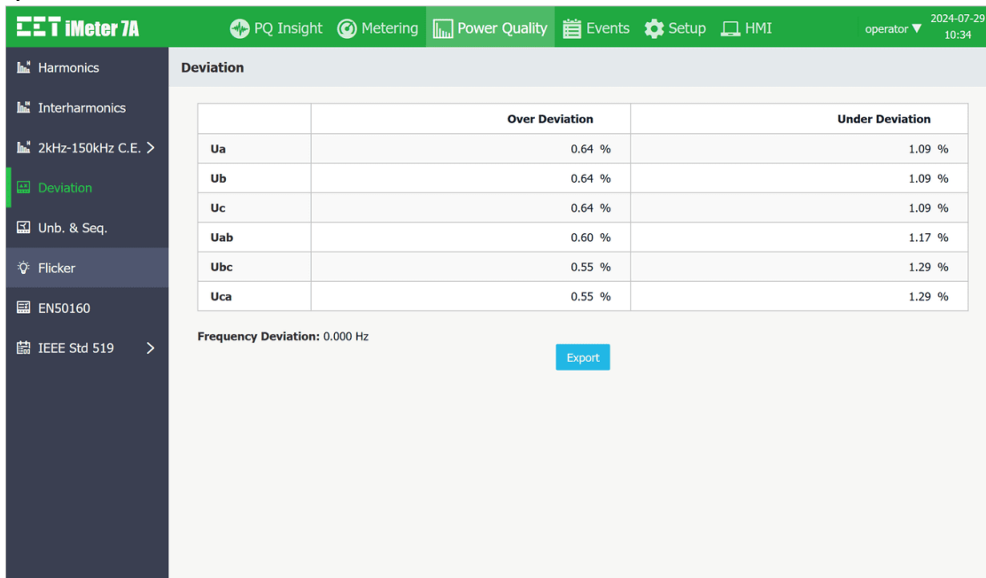
Figure 3-89 Deviation Interface
