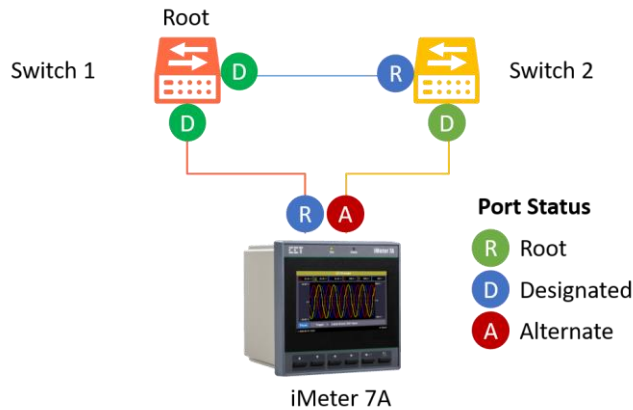
Figure 2-12 Ethernet RSTP Mode
