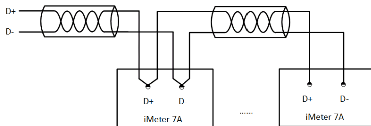
Figure 2-13 RS-485 Communication Connections
