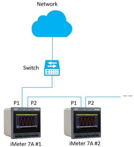
Figure 2-11 Ethernet Normal Mode and Switch Mode
