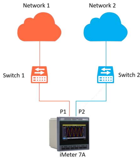
Figure 2-11 Ethernet Normal Mode and Switch Mode
