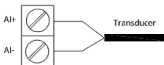
Figure 2-22 Analog Input Wiring
