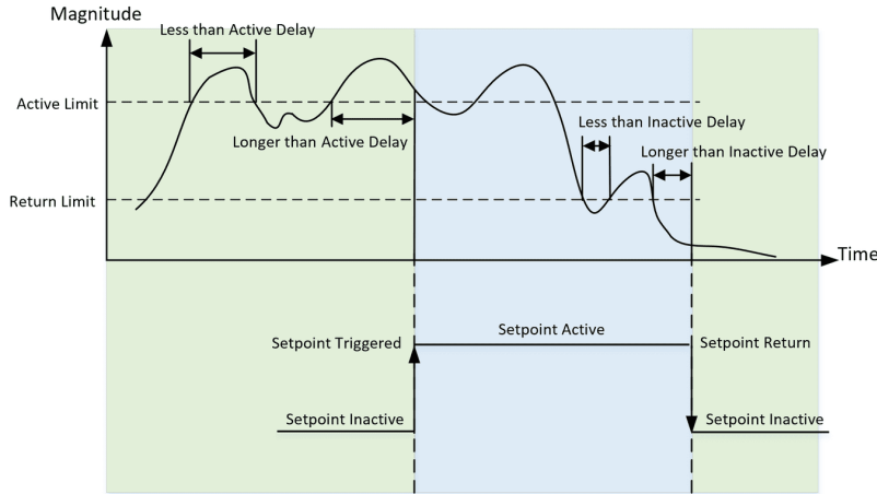
Figure 4-25 Over Setpoint
