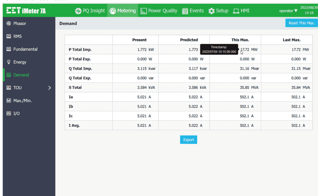
Figure 3-75 Demand Interface
